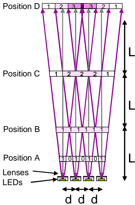
Figure 3 Schematic of Gradual Expanding Beams
