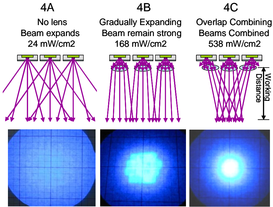
Figure 4 Comparison of LED Far Field Pattern
