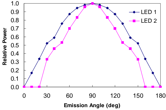
Figure 2 Far Field Pattern of UV LEDs
