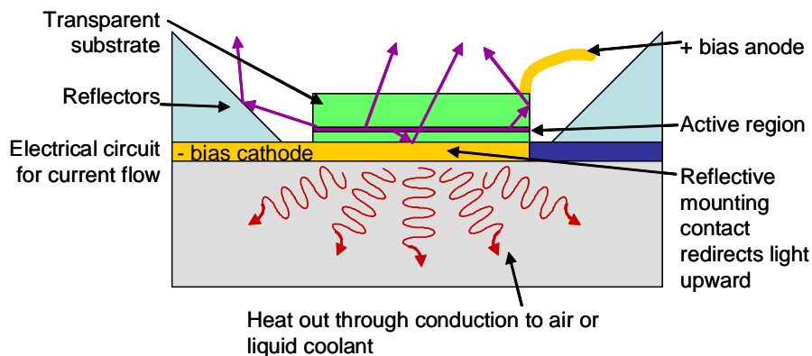
Figure 1. Cross section of a typical UV LED.
