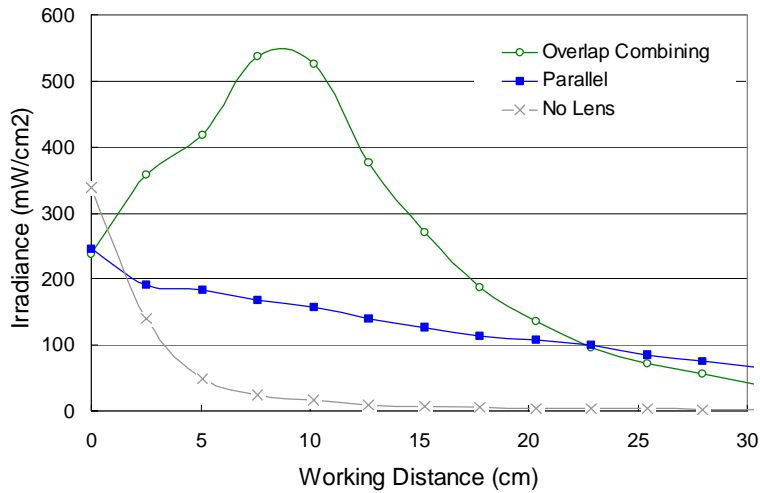
Figure 5 Graph of Irradiance vs. Working Distance
