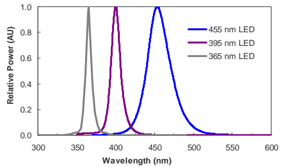
LED Spectrum
